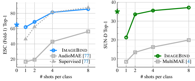
Figure 3. Few-shot classification on audio and depth. We report the emergent zero-shot classification performance on each benchmark (denoted by \star ). We train linear classifiers on fixed features for the \geq 1 -shot case. (Left) In all settings, IMAGEBIND outperforms the self-supervised AudioMAE model. IMAGEBIND even outperforms a supervised AudioMAE model upto 4 shot learning showing its strong generalization. (Right) We compare with the MultiMAE model trained with images, depth, and semantic segmentation masks. IMAGEBIND outperforms MultiMAE across all few-shot settings on few-shot depth classification.
